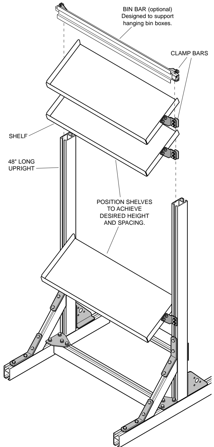
Figure 8. ATTACHING SHELVES
