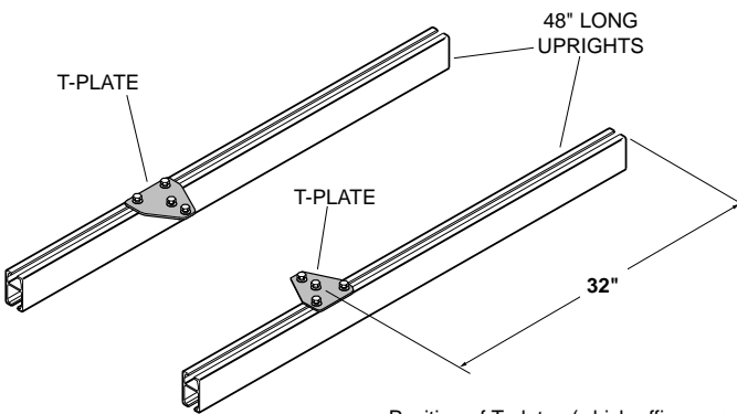
Figure 3. ASSEMBLING FRAME UPRIGHTS
