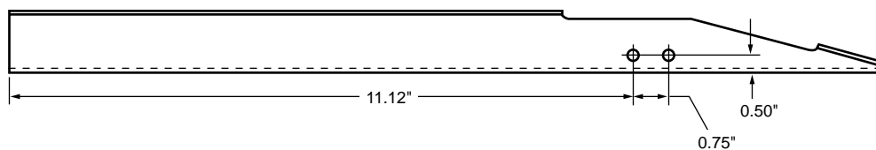
Figure 2-KEYBOARD BRACKET HOLE LOCATION
