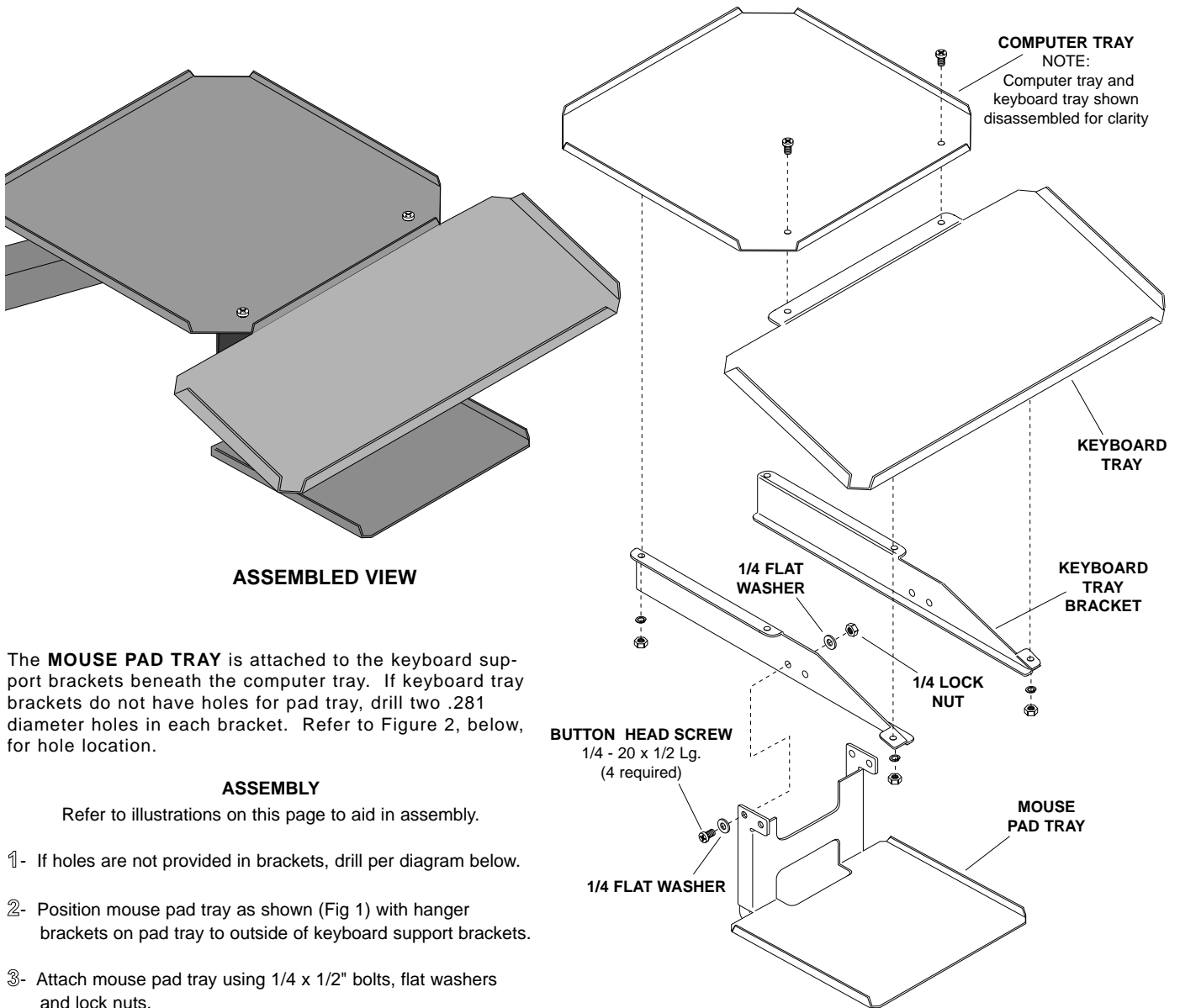
Figure 1-COMPUTER, KEYBOARD AND MOUSE PAD TRAYS
