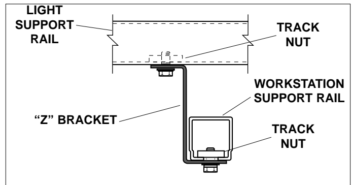
Figure 2-END VIEW
